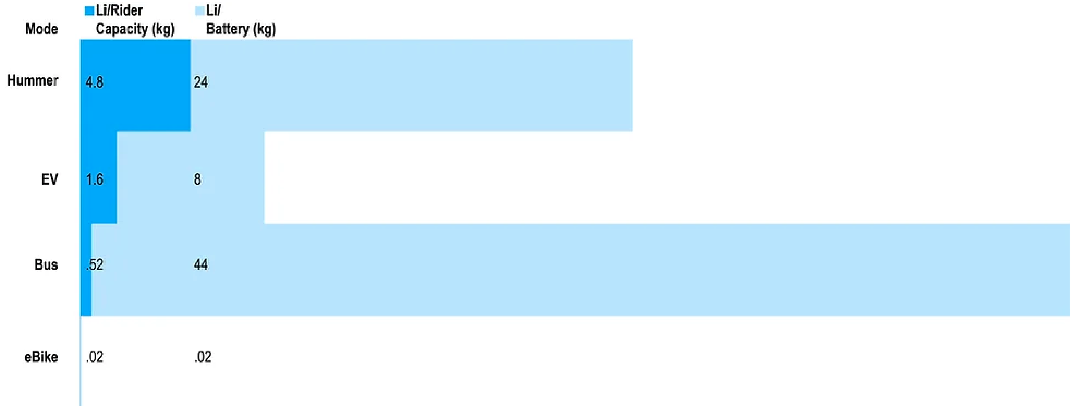
A comparative chart of e-Hummer, EV, e-bus, and e-bike lithium intensities.
